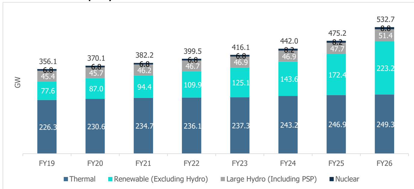
Chart 13: Installed Capacity Trend
