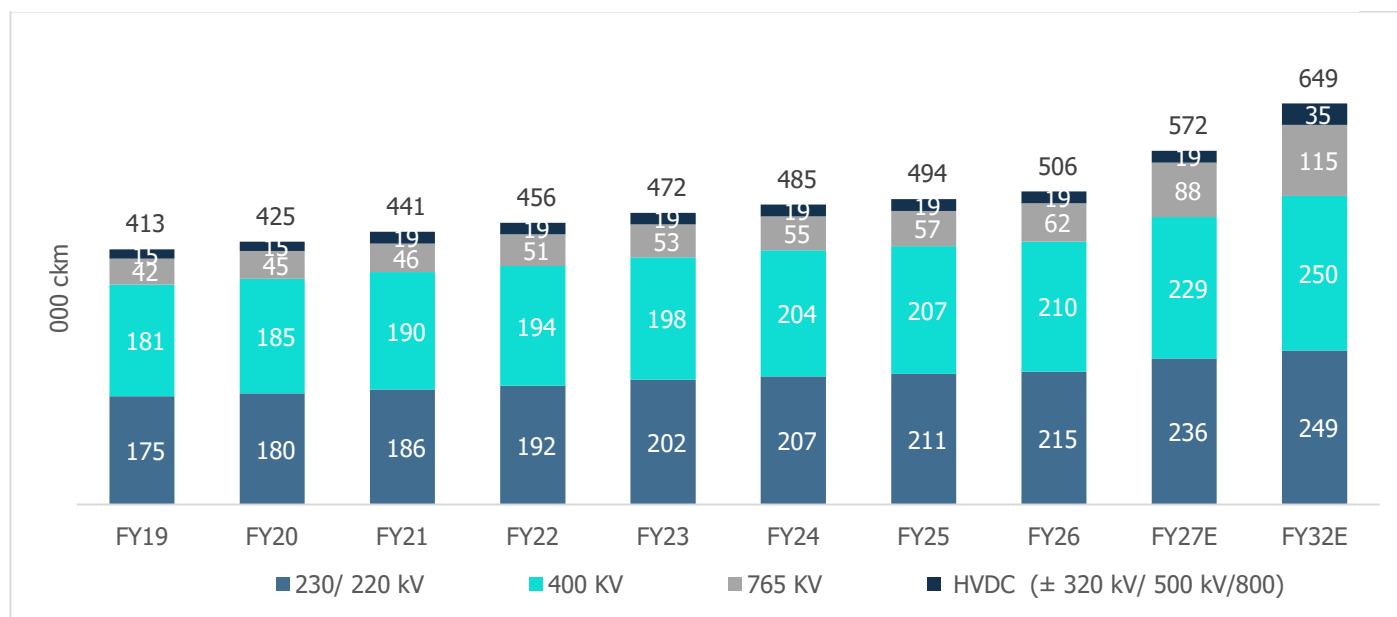
Chart 25: Transmission Line Network (220 kV & above)
