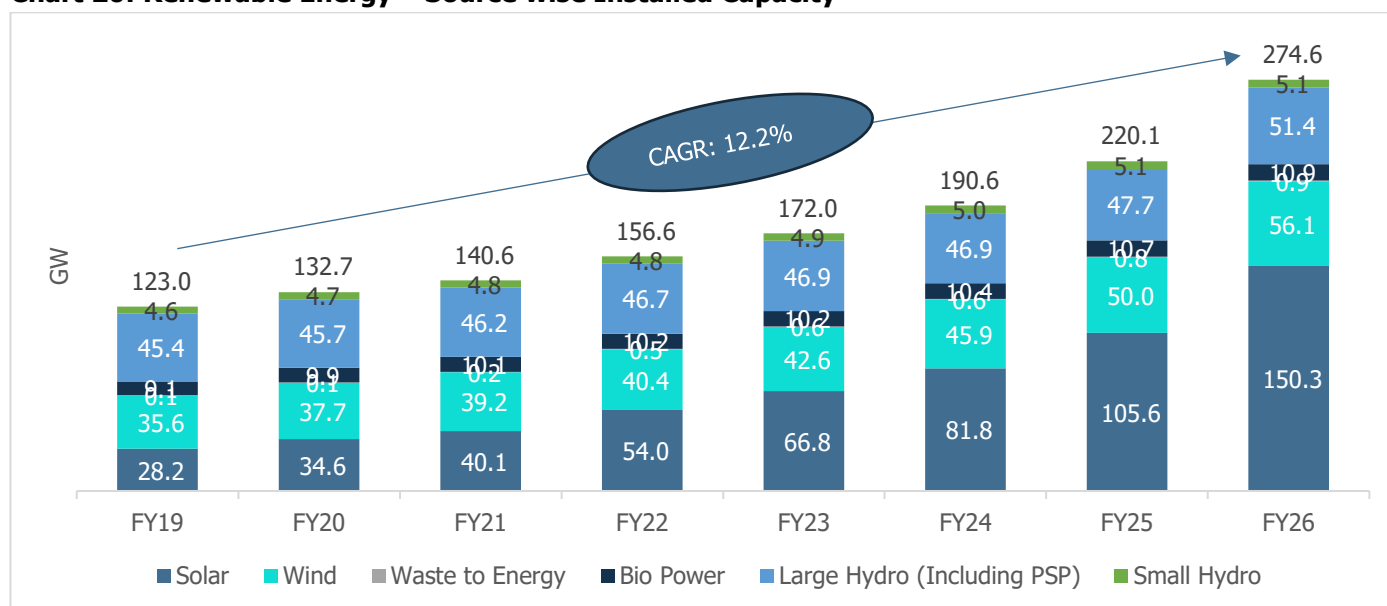
Chart 20: Renewable Energy – Source wise Installed Capacity
