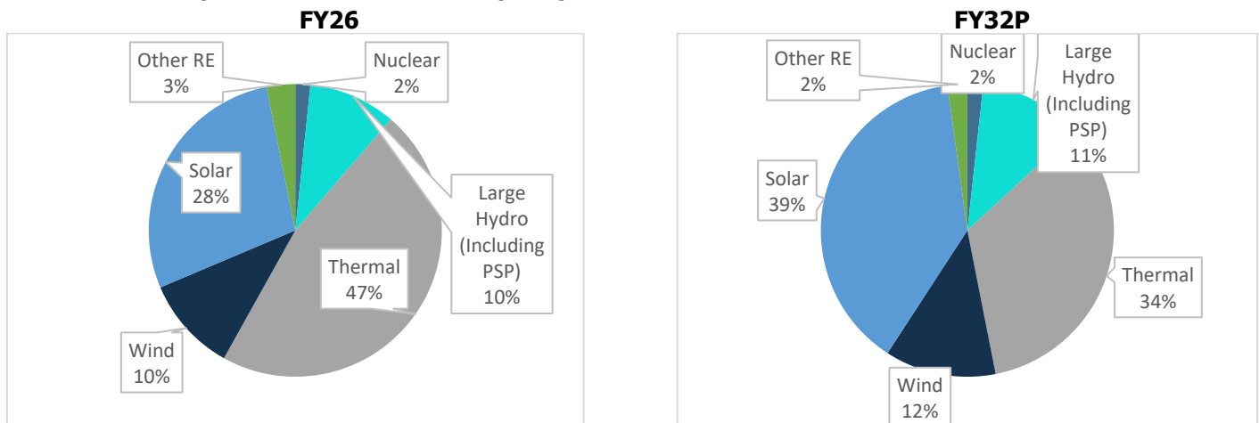
Chart 18: Break-up of the total installed capacity - FY26 vs FY32P
