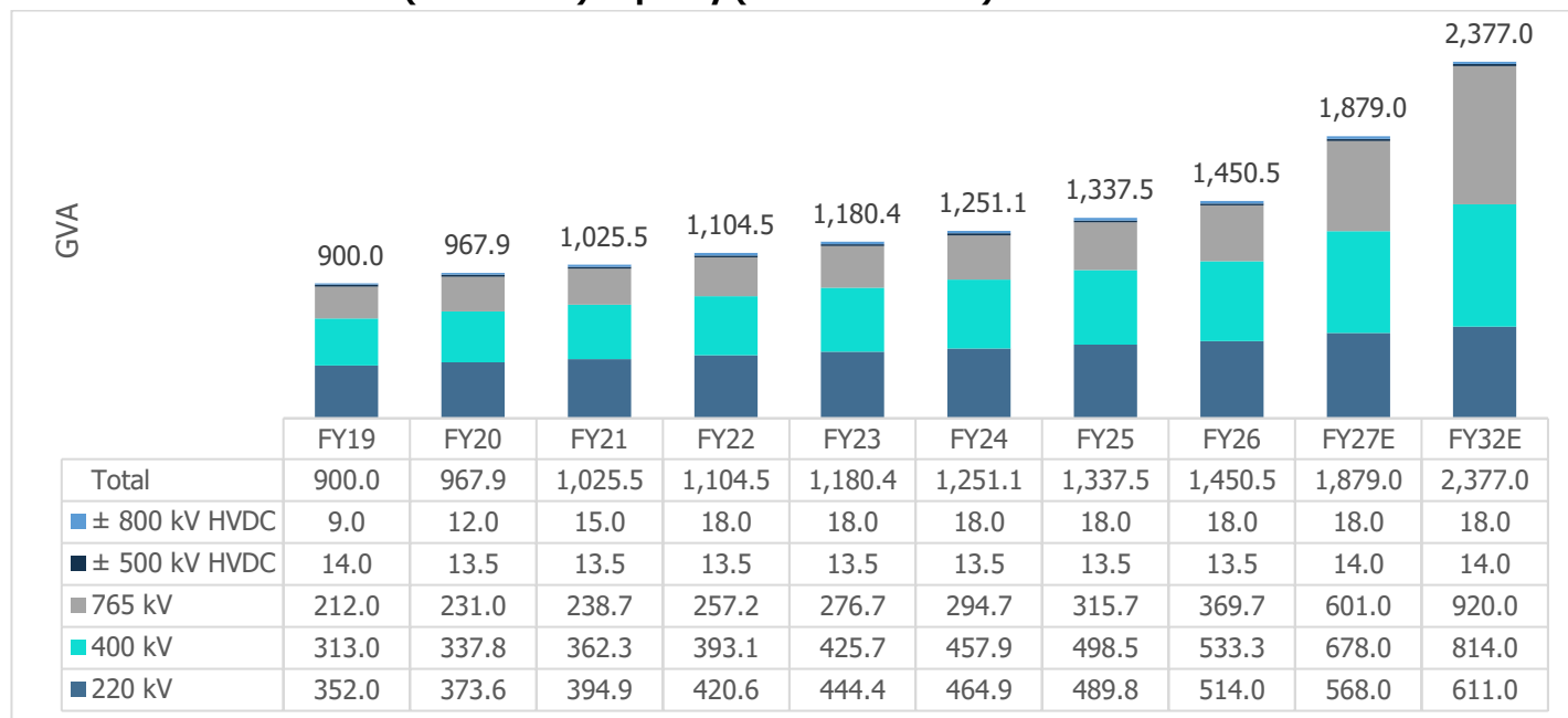
Chart 26: Transformation (Substation) Capacity (220 kV & Above)
